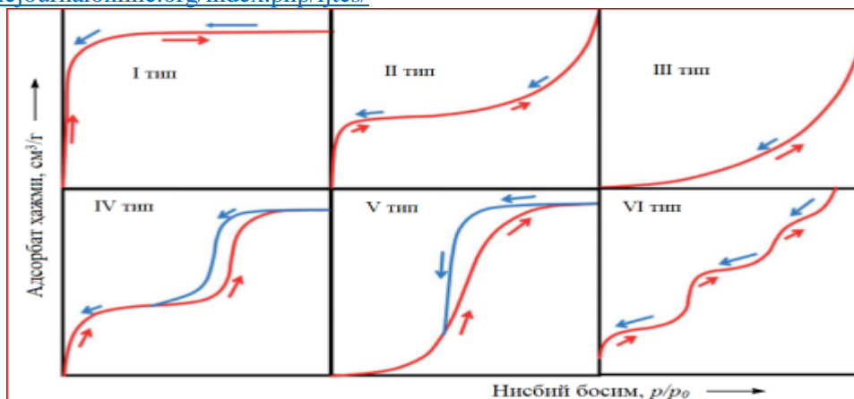
1-picture. Types of isotherms of sorbts from adsorption of various gases into sorbents.
