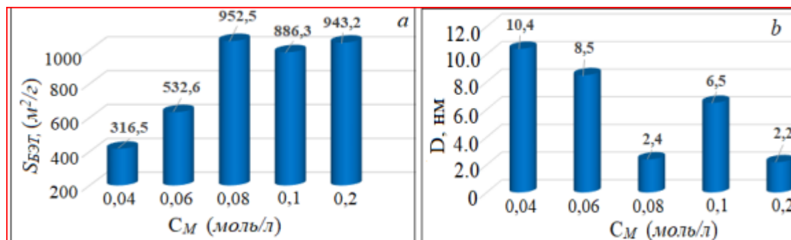
2-picture. The relative surface (a) of Kremnezem sorbent and the dependence of the size of the pores (b) on the concentration of the Teos.
